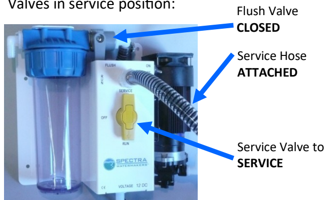
Valves in service position:
